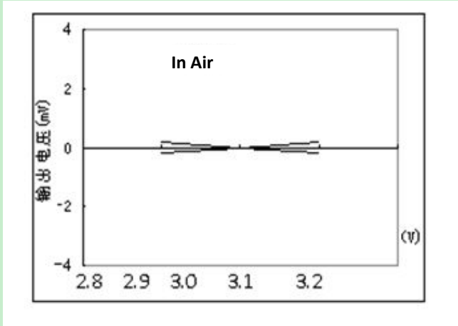
Fig9. Zero point with different voltage
