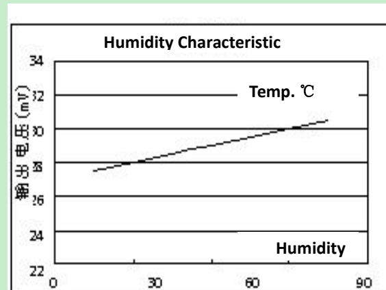
Fig8. Sensitivity at different humidity
