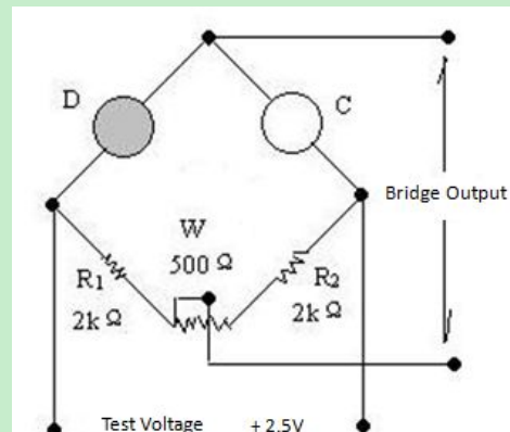
Fig1.Sensor structure
