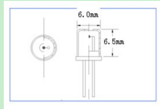
Fig1.Sensor structure
